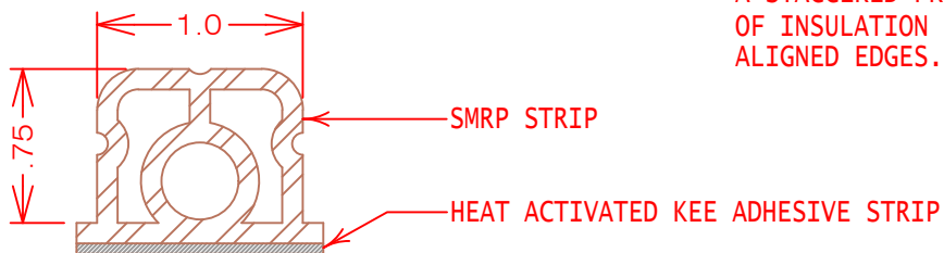
SMRP SECTION VIEW
