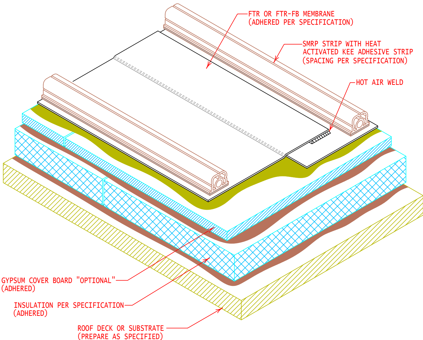
SMRP SECTION VIEW
