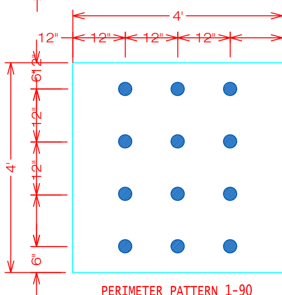
PERIMETER PATTERN 1-90 NON-HURRICANE ZONE 4' X 8' = 24 PER BOARD 4' X 4' = 12 PER BOARD
